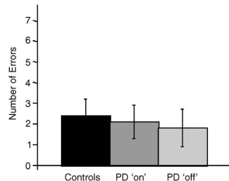
Fig. 4. Mean number of errors for subjects in each group on the last ‘retraining’ phase of the task.
